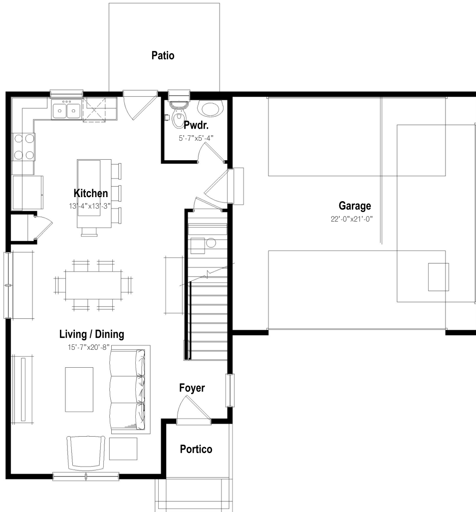
FIRST FLOOR
